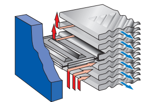
Cross-section of a baffle arrangement illustrating flow distribution
